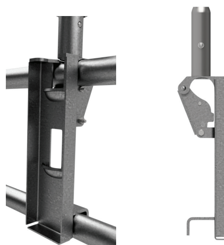
Locking Intermediate Horizontal Adapter (2011–2015, Run 46 – Run 55)
