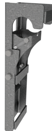
Locking Intermediate Horizontal Adapter for Outer Deck (2016–Present, Run 57 – Run 60)
